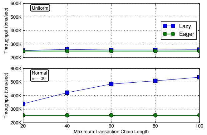
Figure 3: Microbenchmark Throughput
